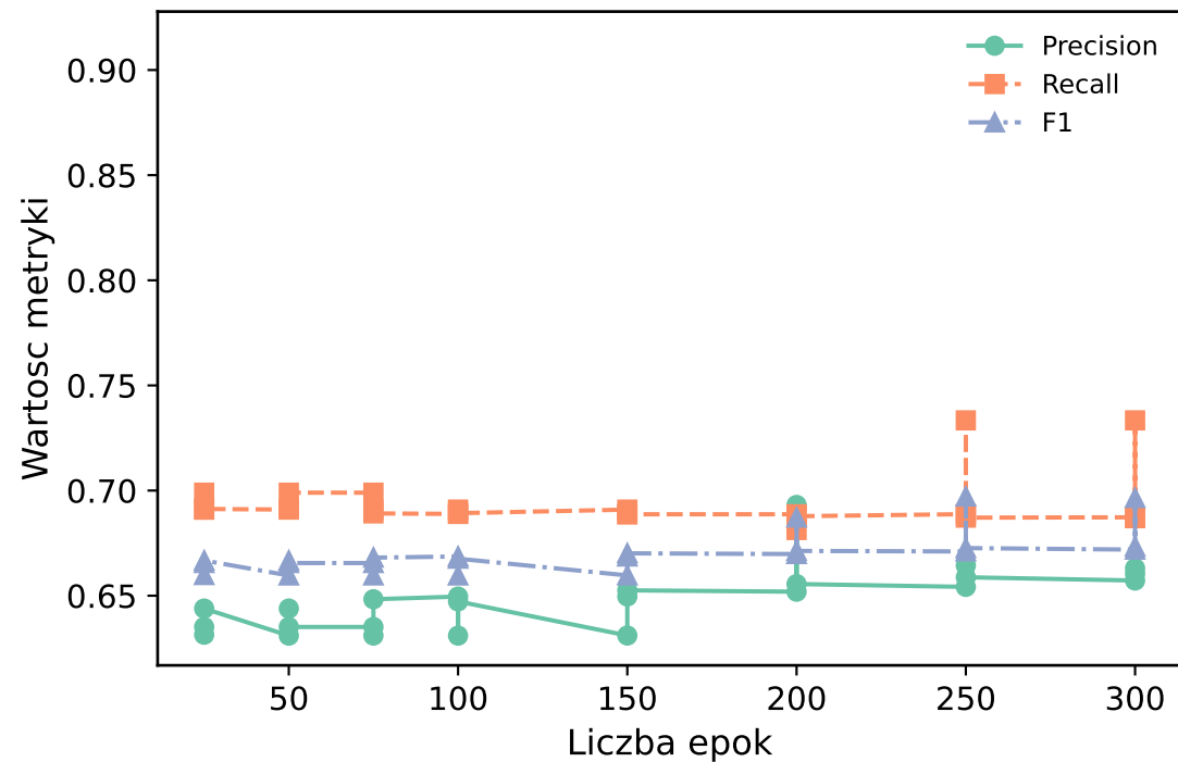
CICIDS 2017
