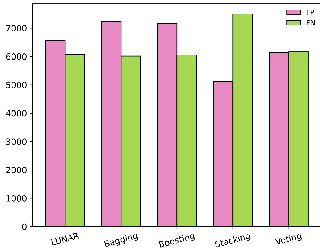
CICIDS 2017
