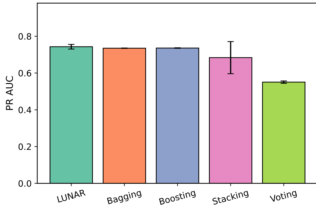
CICIDS 2017
