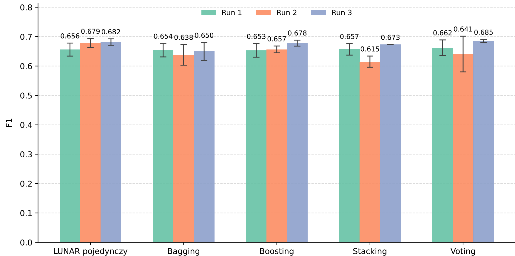
F1: self-ensemble LUNAR vs LUNAR pojedynczy — CICIDS2017
