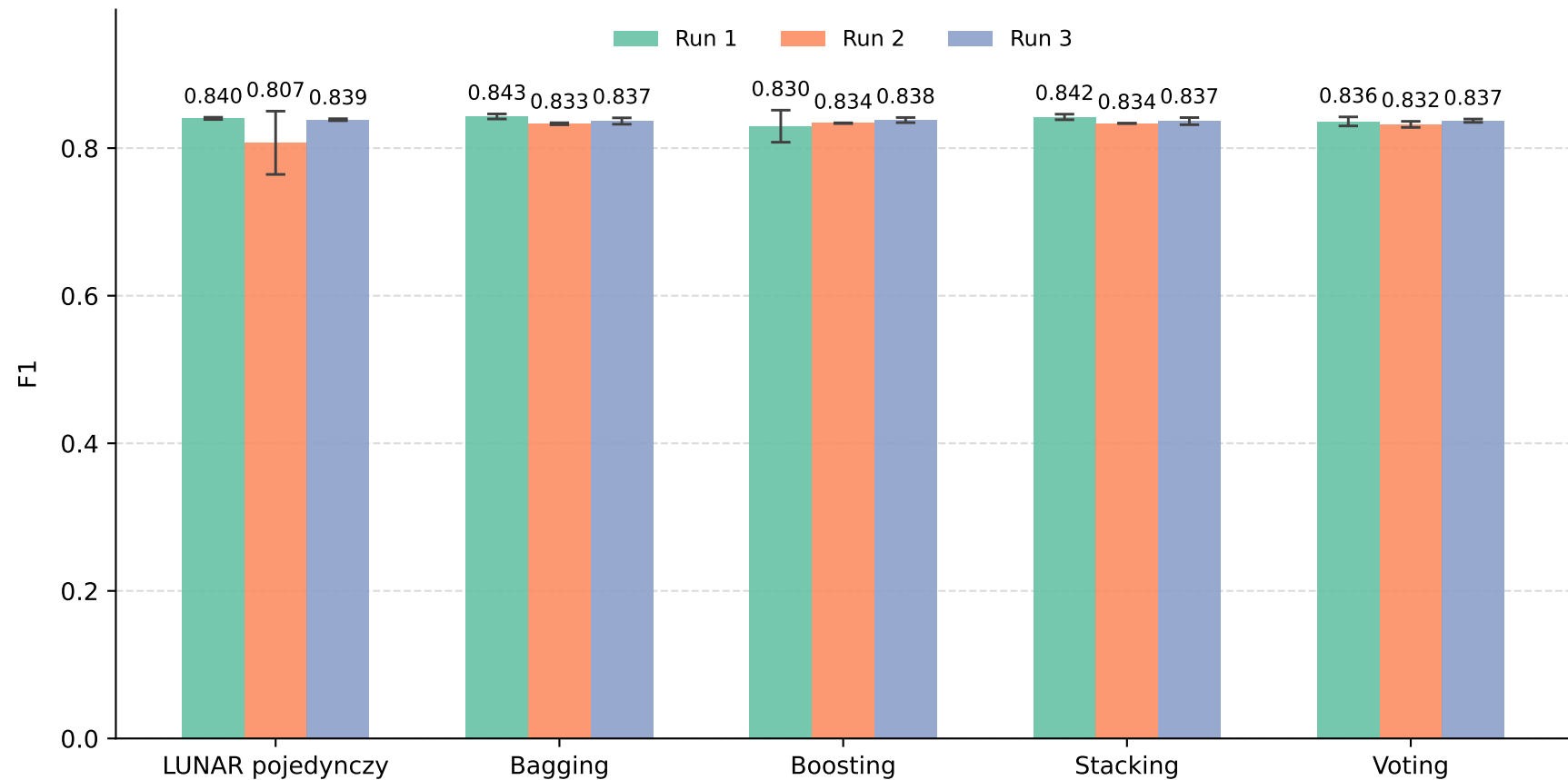
F1: self-ensemble LUNAR vs LUNAR pojedynczy — UNSW-NB15
