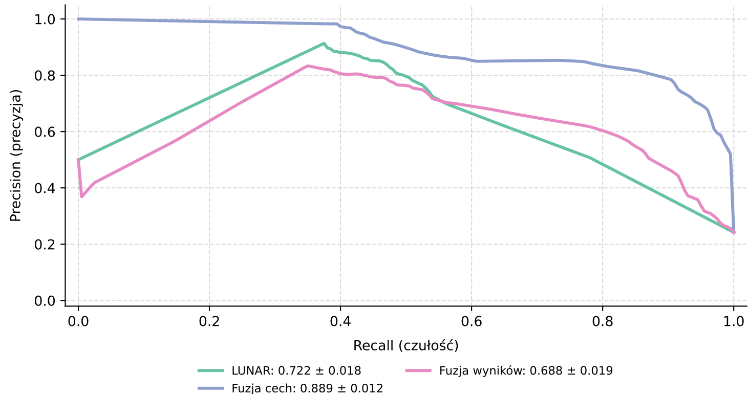
Krzywe precision-recall: CICIDS2017 — Run 1
