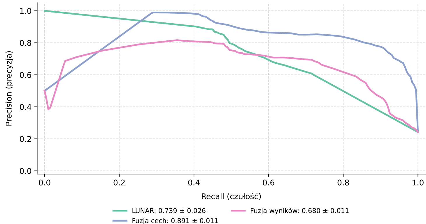
Krzywe precision-recall: CICIDS2017 — Run 2
