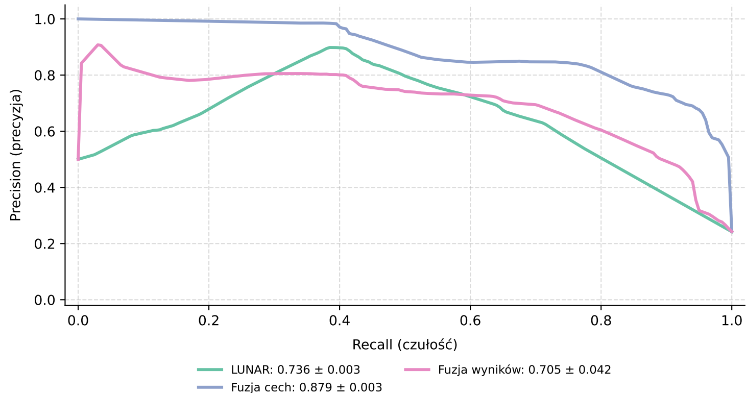
Krzywe precision-recall: CICIDS2017 — Run 3
