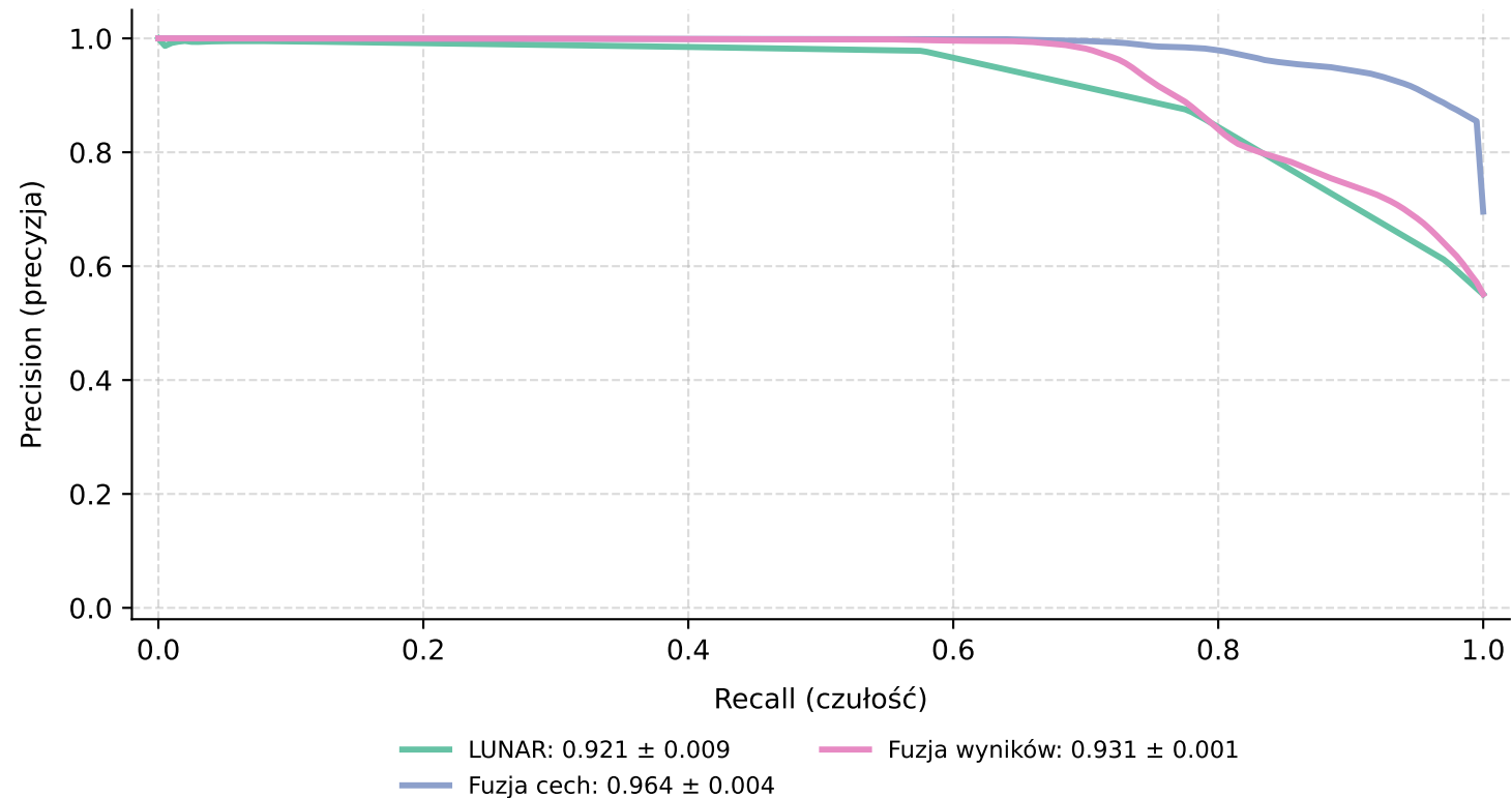
Krzywe precision-recall: UNSW-NB15 — Run 1
