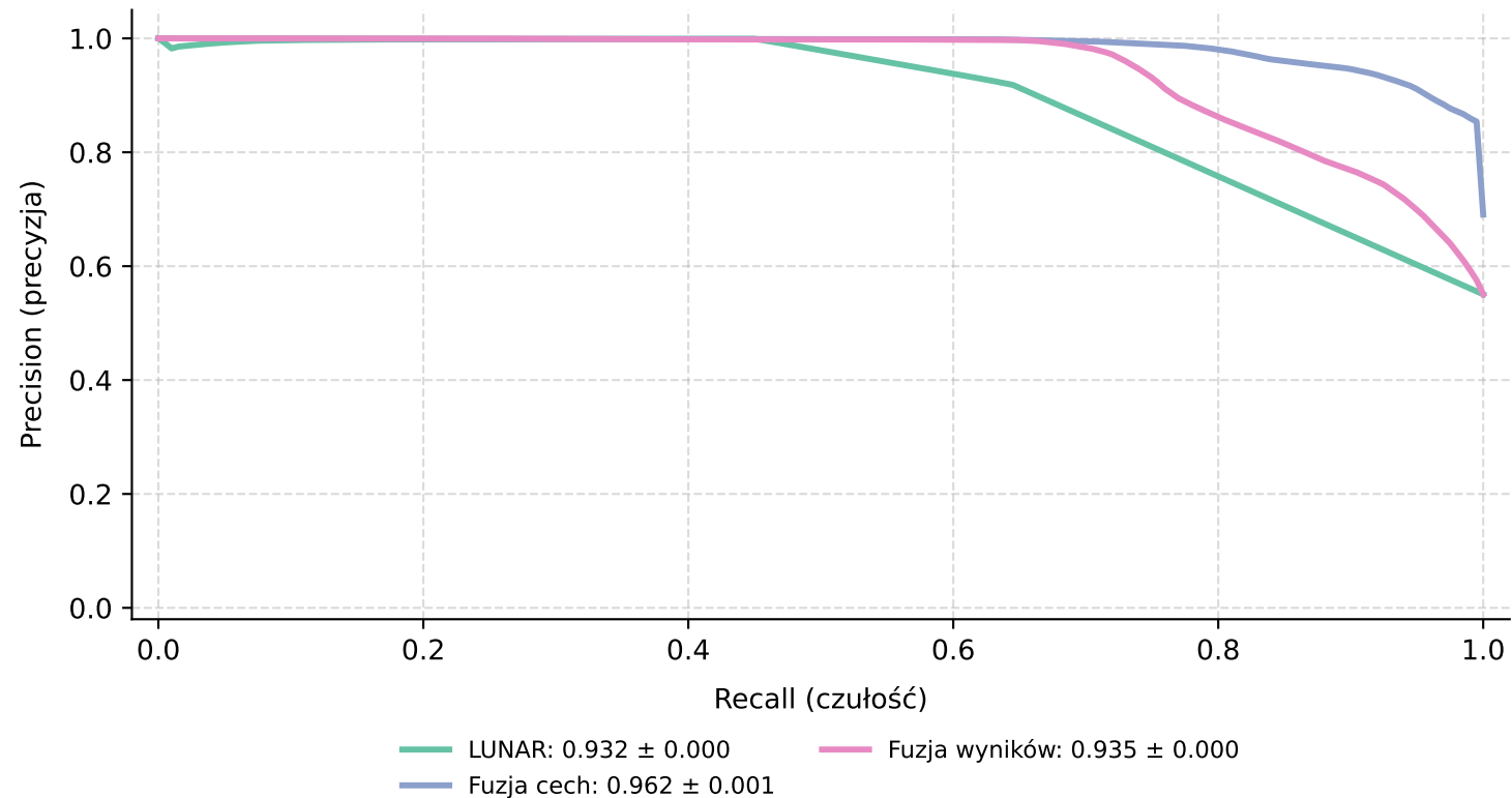
Krzywe precision-recall: UNSW-NB15 — Run 2
