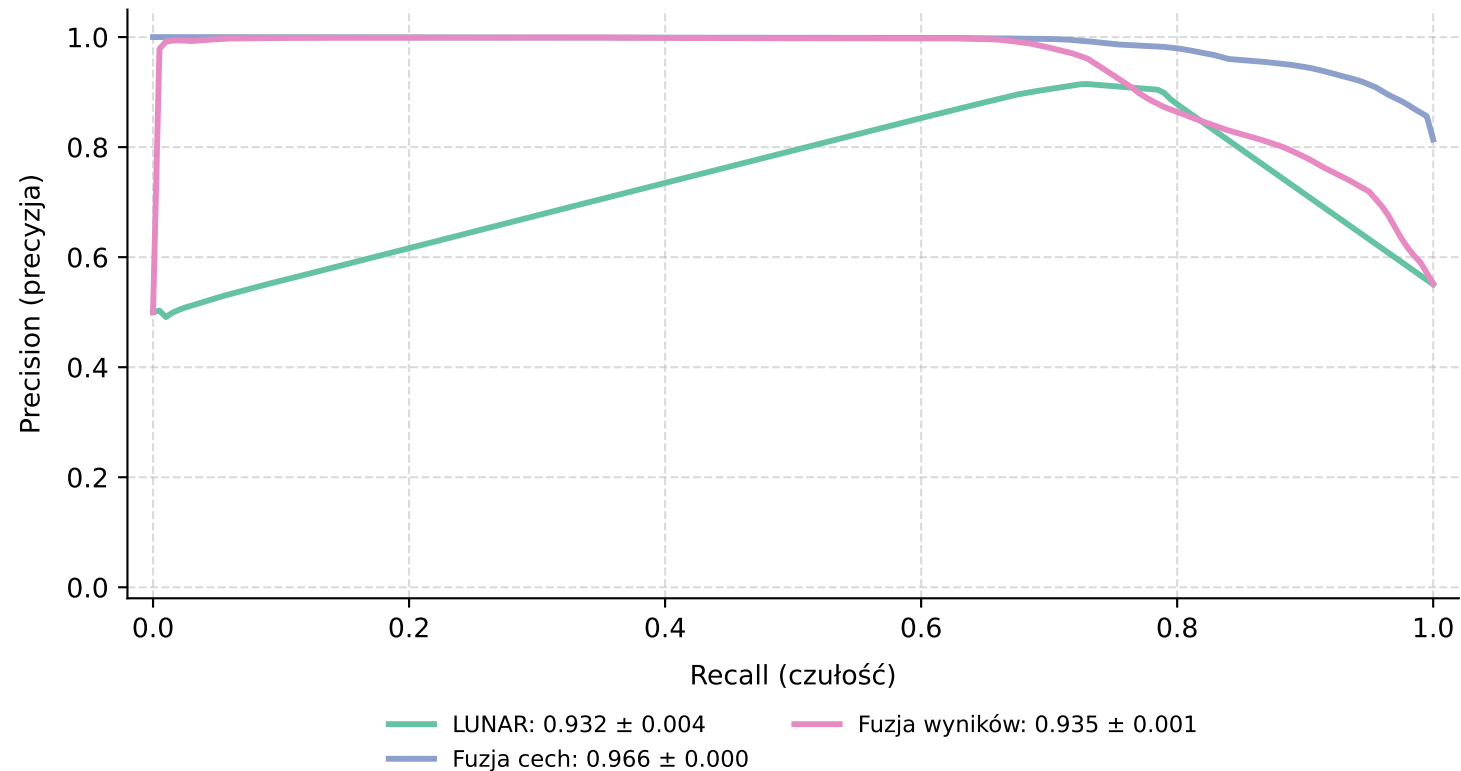
Krzywe precision-recall: UNSW-NB15 — Run 3
