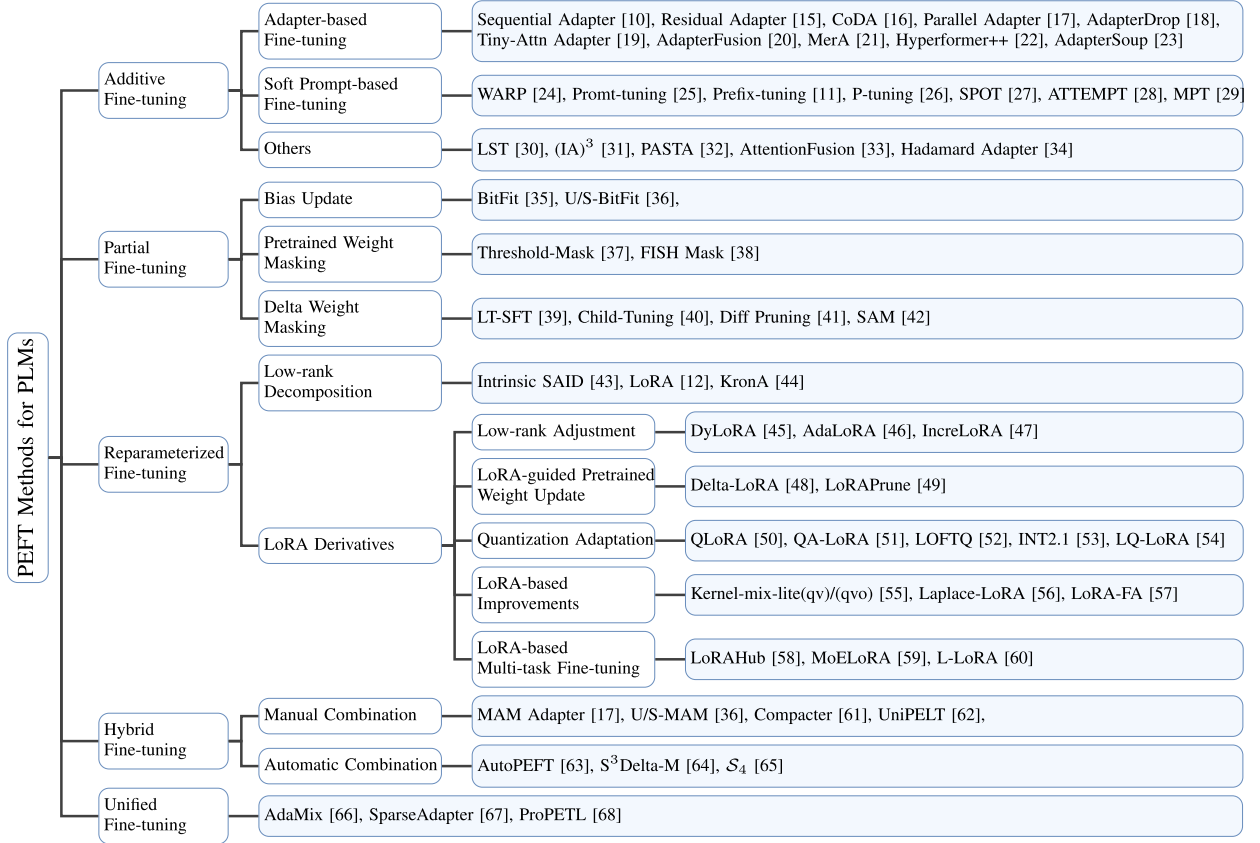
Fig. 2. Taxonomy of PEFT Methods for PLMs in NLP. Based on their characteristics, PEFT methods are categorized into five main categories: Additive Fine-tuning, Partial Fine-tuning, Reparameterized Fine-tuning, Hybrid Fine-tuning, and Unified Fine-tuning. Each category encompasses various approaches, such as adapter-based, soft prompt-based, and other fine-tuning methods under Additive Fine-tuning.
