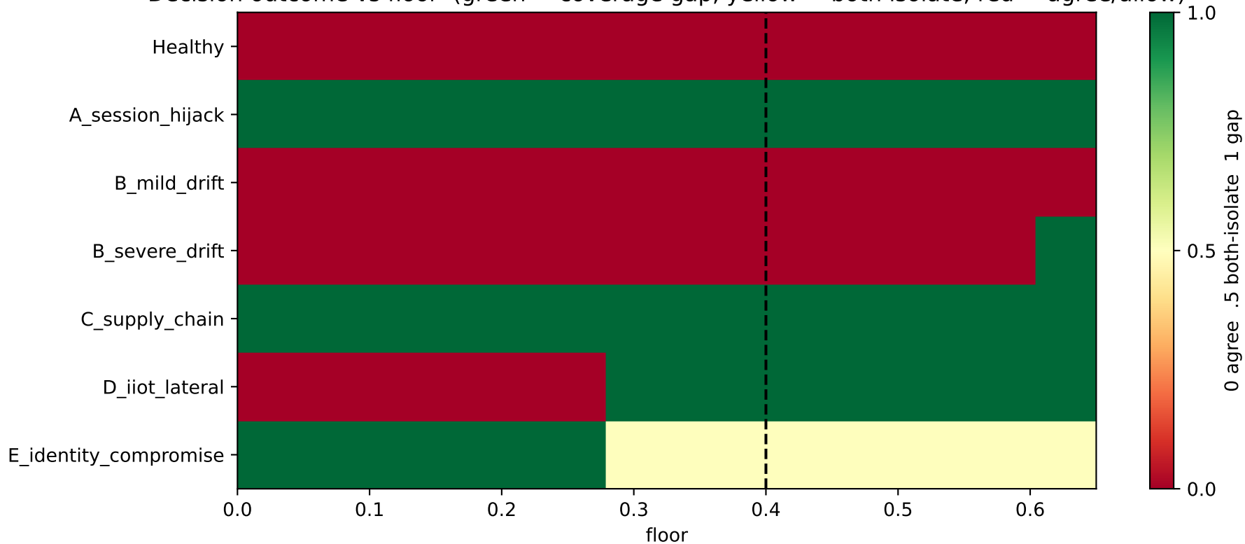
Decision outcome vs floor (green = coverage gap, yellow = both isolate, red = agree/allow)
