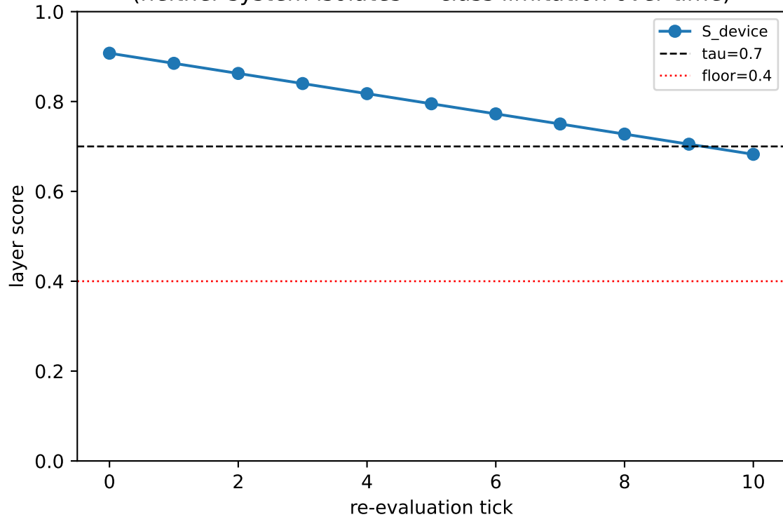
B: device posture drift (neither system isolates — class limitation over time)
