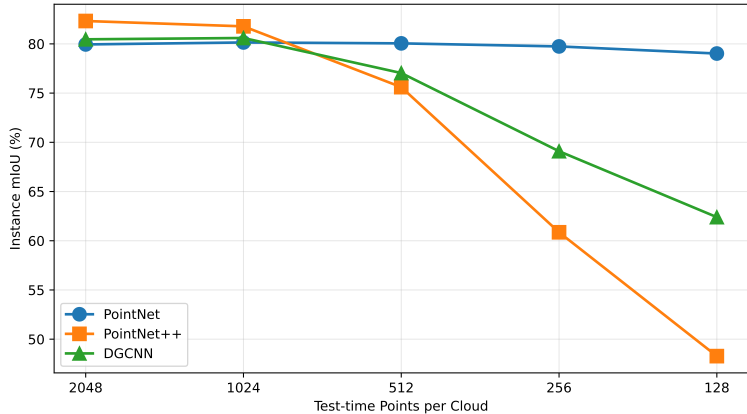
Robustness to Test-Time Point Cloud Density (all models trained at 2048 points)
