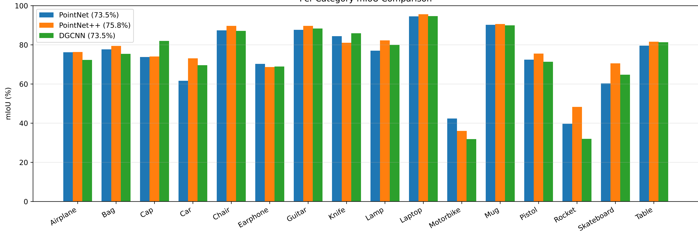
Per-Category mIoU Comparison
