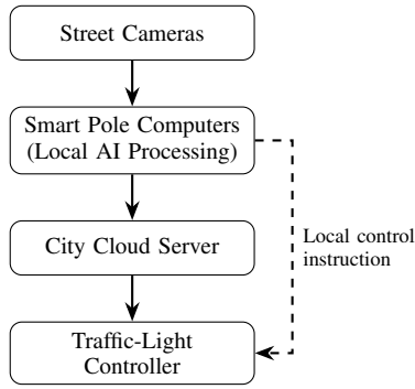
Fig. 2. Architecture of the local AI-based traffic system.
