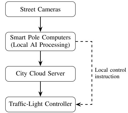
Fig. 1: Architecture of the local AI-based traffic system
