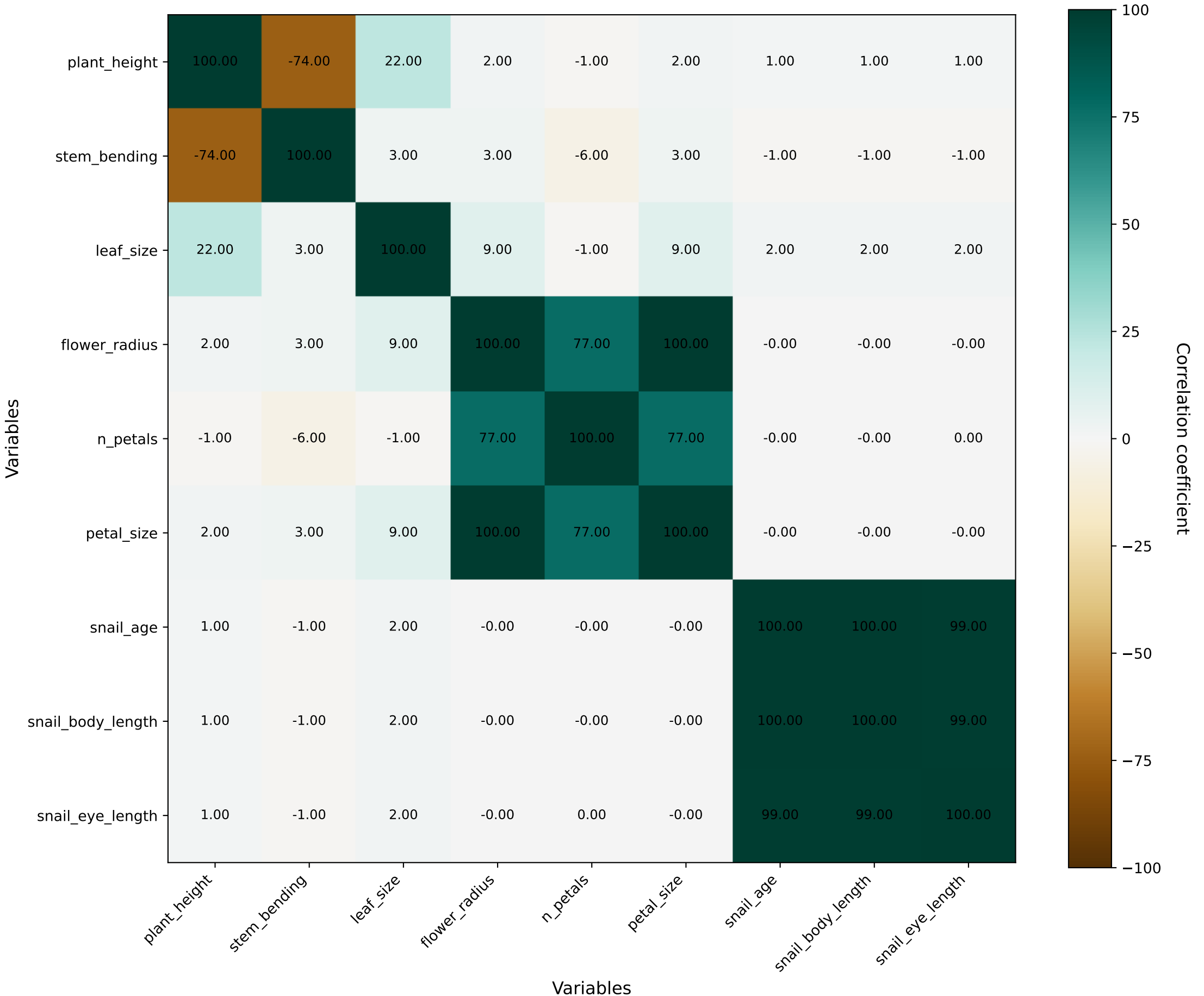
Spearman correlation between features
