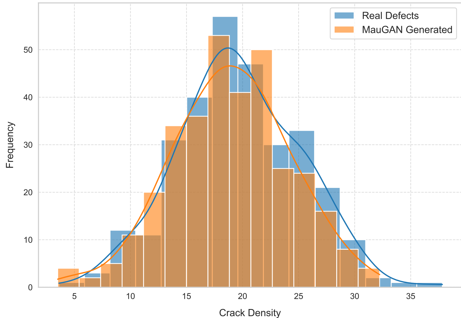
Glass Breakage Crack Density (cracks/100 cm 2 )
