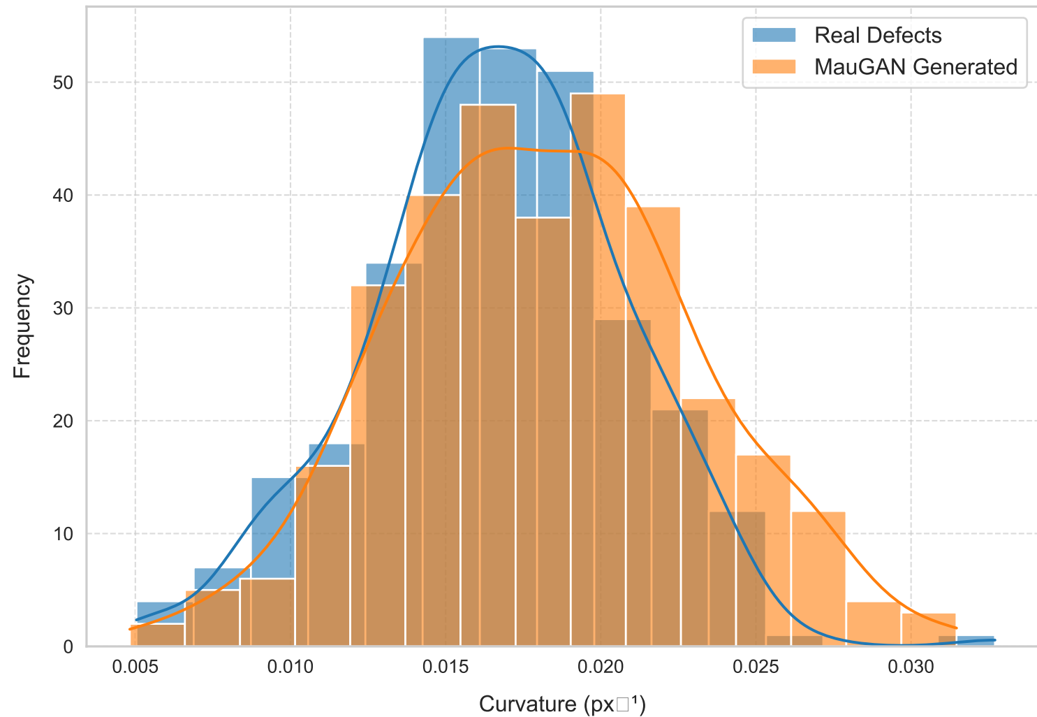
Microcrack Median Curvature ( \text{px}^{-1} )
