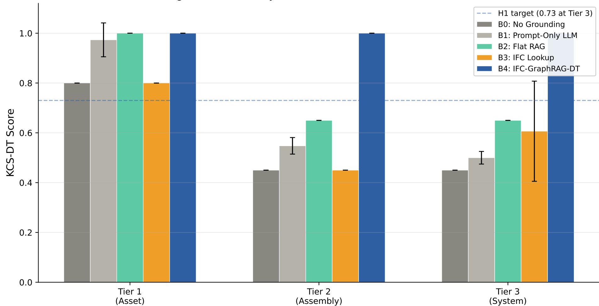
Figure 1: KCS-DT by Baseline and Tier (DTAH-Bench-50)
