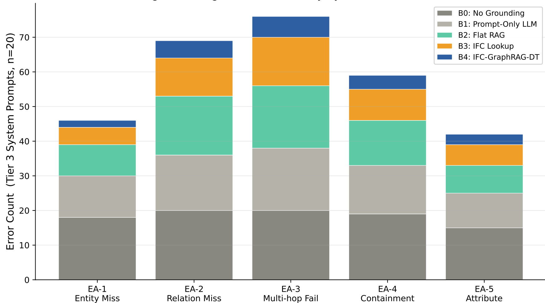
Figure 4: Stage A Error Taxonomy by Baseline — Tier 3
