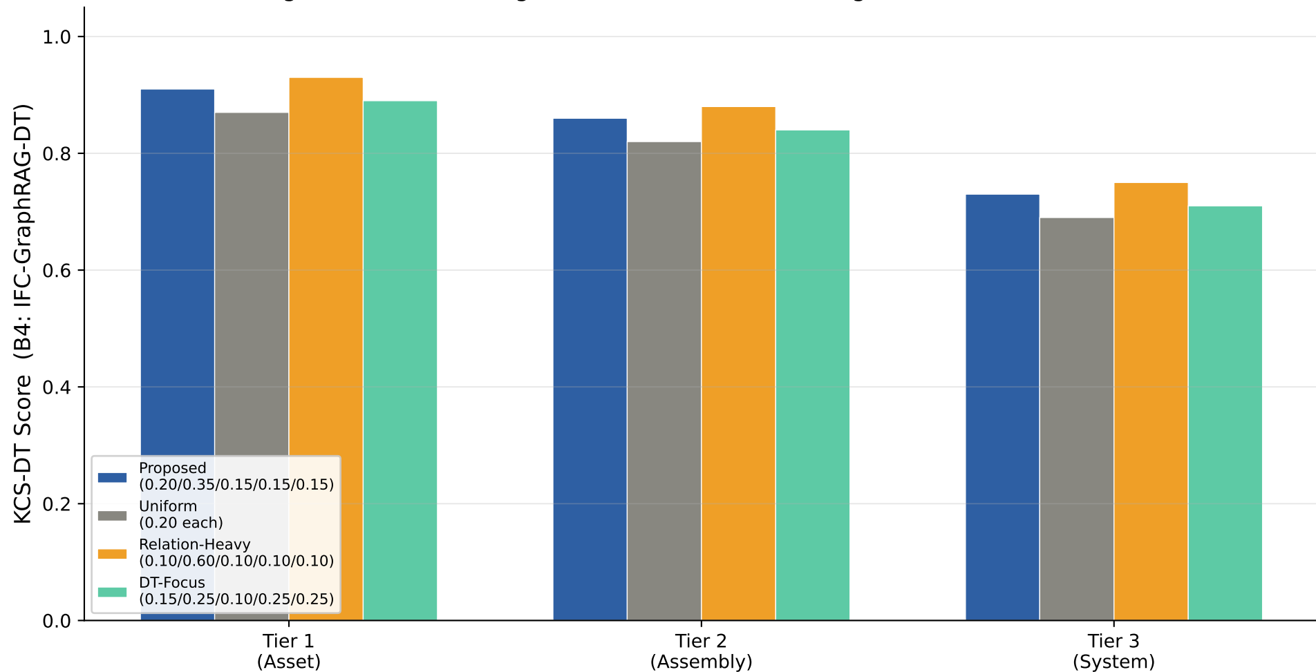
Figure 5: KCS-DT Weight Ablation — Effect of Weight Vector on B4 Scores
