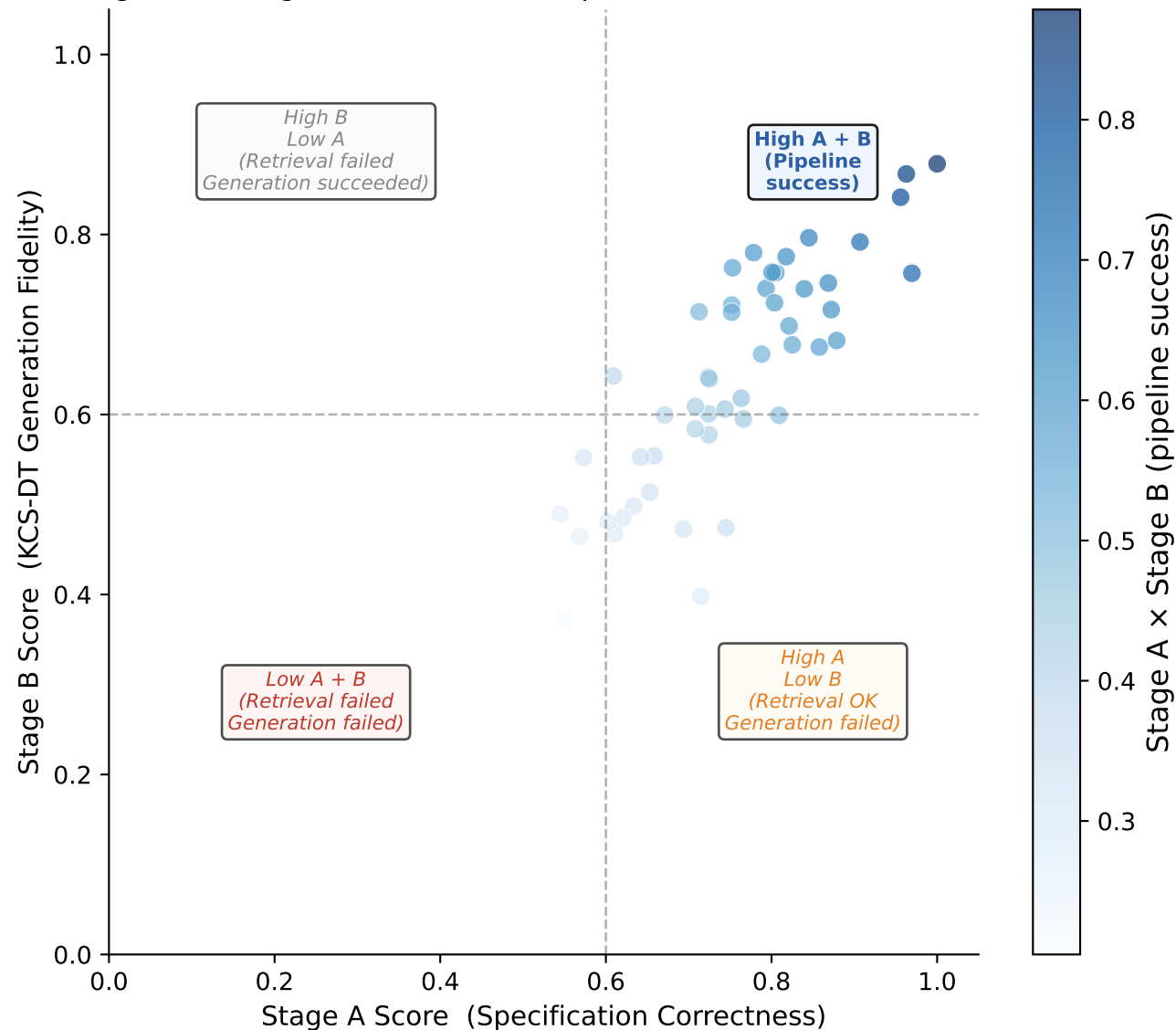
Figure 7: DTAH-Eval Two-Stage Diagnostic Stage A vs Stage B failure mode separation (B4, DTAH-Bench-50)
