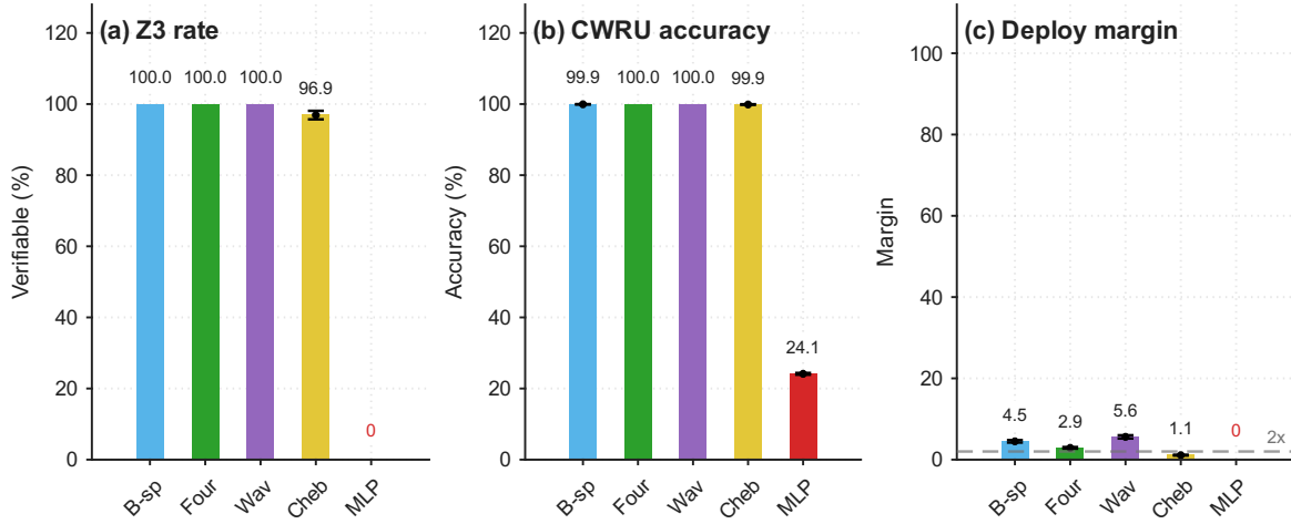
Fig. 3. C^2 -BV Architecture Family: SVNN Verification Across 5 Architectures. Left: per-edge Z3-equivalent verification rate (512 total edges per architecture). All four C^2 -BV architectures (B-spline, Fourier, Wavelet, ChebyKAN) achieve \geq 96.9\% Z3 verification; standard MLP achieves 0/48 (E41). Right: CWRU test accuracy and Z3 safety margin (ratio of the per-function margin to \max M_2 \cdot h^2 / 8 ). WaveletKAN's wide margin reflects M_2 -regularized training ( \lambda = 0.01 ). FourierKAN's M_2 is bounded by \omega^2 \sum k^2 (|c_k| + |d_k|) (Proposition 6(c)). Safety margins \geq 2\times confirm deployability for all C^2 -BV architectures.
