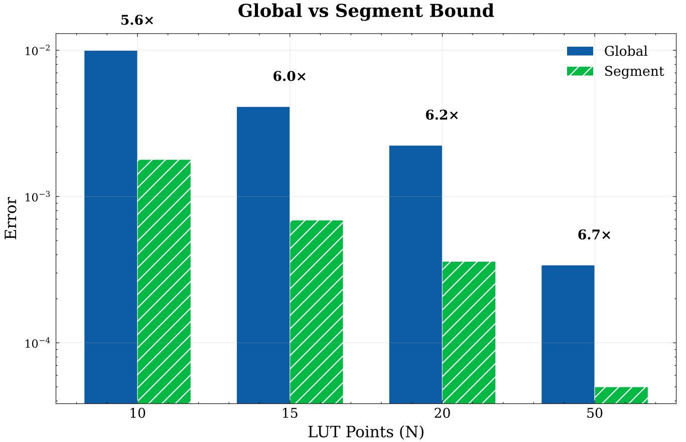
Fig. 10. Segment-Aware Bound Comparison Across LUT Resolutions. (a) Global vs. per-segment worst-case error: segment-aware M_{2,j} achieves 6.0× mean tightening across all resolutions. (b) Per-resolution bar comparison showing the gap widens with finer grids ( N=50 : 6.7×). (c) Segment coverage: > 96% of LUT segments have error < 50% of the global bound; 67–72% have error < 20% of global. The dashed line shows the monotonic improvement with LUT resolution N .
