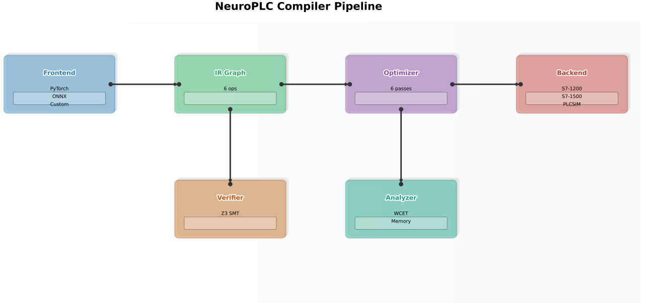
Fig. 6. Compiler architecture. Four-stage IR-based pipeline: Frontend (PyTorch \rightarrow IR) \rightarrow IR Graph (6 operation types) \rightarrow Optimizer (adaptive B-spline LUT) \rightarrow Backend (SCL code generation for S7-1200/S7-1500).
