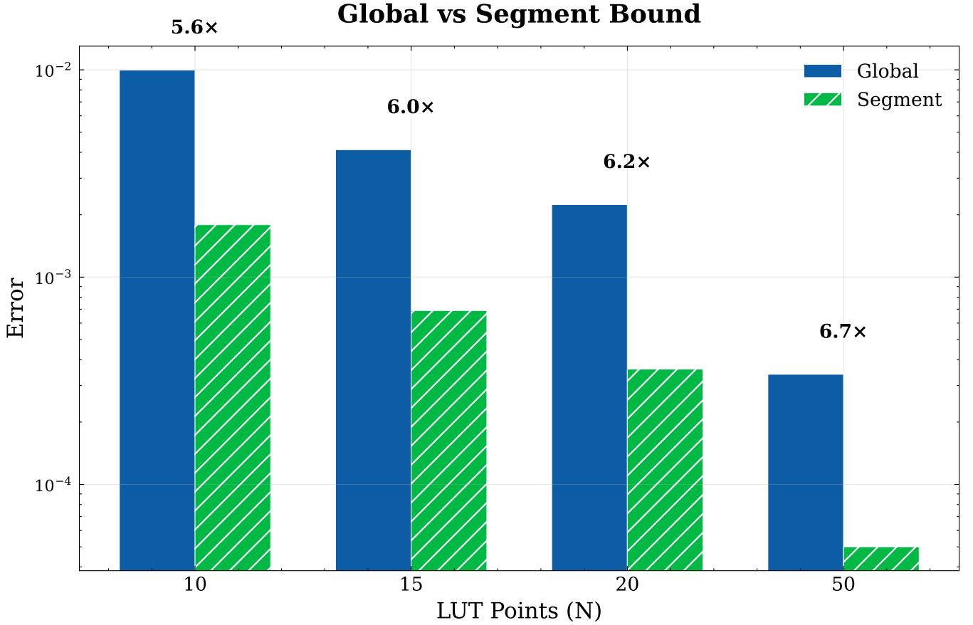
Fig. 10. Segment-Aware Bound Comparison Across LUT Resolutions. (a) Global vs. per-segment worst-case error: segment-aware M_{2,j} achieves 6.0\times mean tightening across all resolutions. (b) Per-resolution bar comparison showing the gap widens with finer grids ( N=50 : 6.7\times ). (c) Segment coverage: > 96\% of LUT segments have error < 50\% of the global bound; 67\text{--}72\% have error < 20\% of global. The dashed line shows the monotonic improvement with LUT resolution N .
