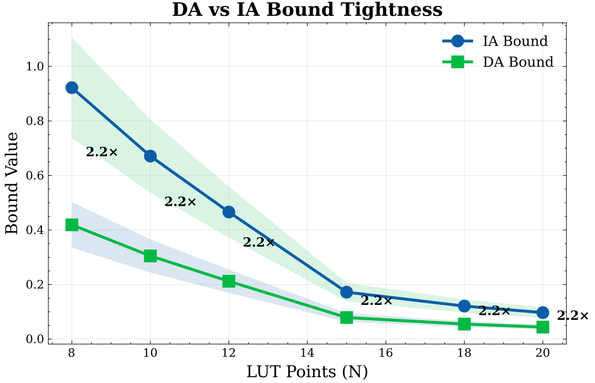
Fig. 9. DA vs. IA Bound Comparison with LUT Resolution. Left: DA achieves 2.2 \times tighter bounds than IA across all LUT resolutions ( N = 8\text{--}20 ), decreasing \propto 1/N^2 (Theorem C). At N=15 : DA = 0.079, IA = 0.172. Right: bar comparison. The gap follows from DA’s Galois-optimality (Theorem B).
