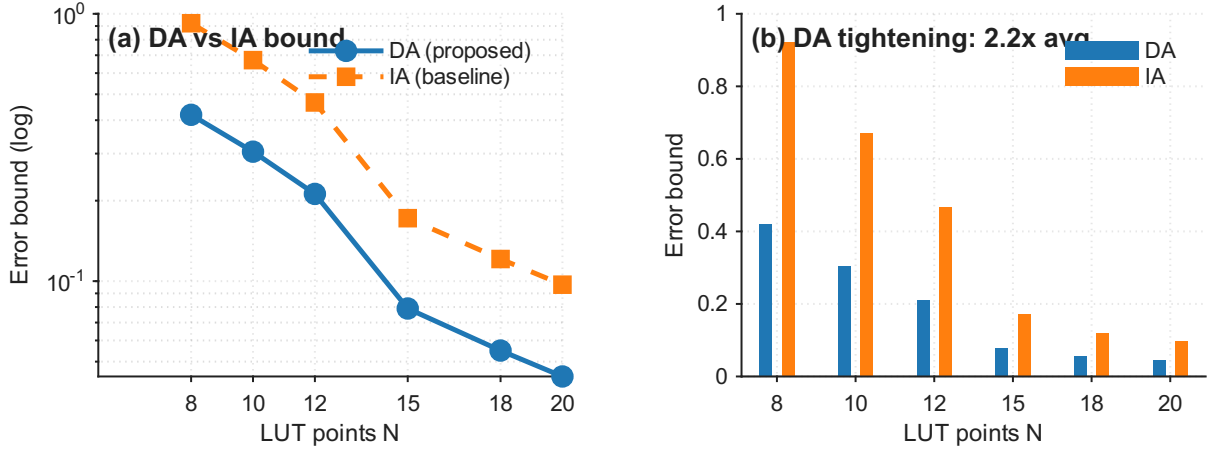
Fig. 9. DA vs. IA Bound Comparison with LUT Resolution. Left: DA achieves 2.2\times tighter bounds than IA across all LUT resolutions ( N = 8\text{--}20 ), decreasing \propto 1/N^2 (Theorem C). At N=15 : DA = 0.079, IA = 0.172. Right: bar comparison. The gap follows from DA's Galois-optimality (Theorem B).
