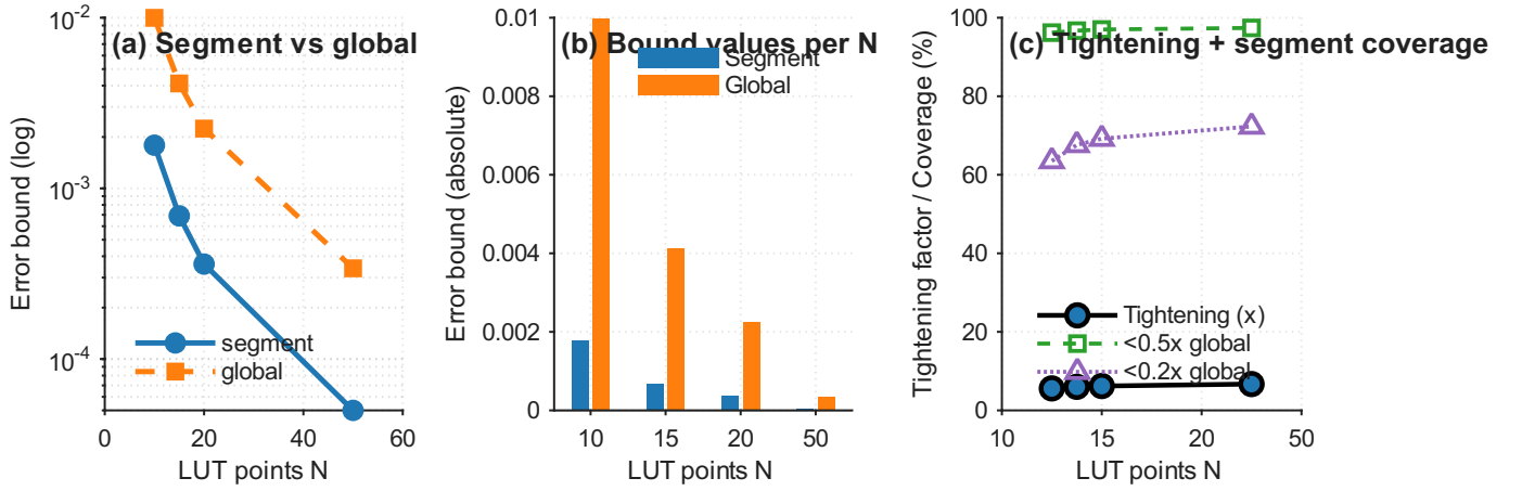
Fig. 10. Segment-Aware Bound Comparison Across LUT Resolutions. (a) Global vs. per-segment worst-case error: segment-aware M_{2,j} achieves 6.0\times mean tightening across all resolutions. (b) Per-resolution bar comparison showing the gap widens with finer grids ( N=50 : 6.7\times ). (c) Segment coverage: > 96\% of LUT segments have error < 50\% of the global bound; 67\text{--}72\% have error < 20\% of global. The dashed line shows the monotonic improvement with LUT resolution N .
