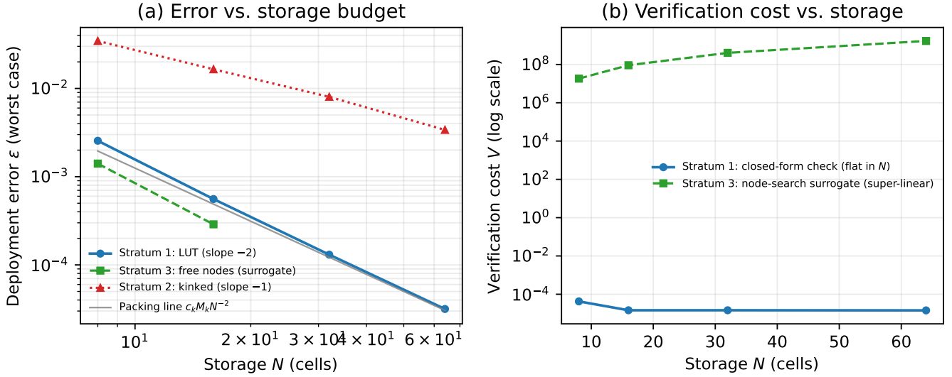
Fig. 1. The verifiable-deployment-capacity plane. (a) Worst-case deployment error vs. storage budget: stratum-1 LUT (slope -2 ), stratum-2 kinked (slope -1 ), stratum-3 free-node surrogate, and the packing line c_k M_k N^{-2} . (b) Verification cost vs. storage: the stratum-1 closed-form check is flat in N (measured wall time), while the stratum-3 structural search grows super-linearly (modeled operation count). Data: E -T4/ E -T5.
