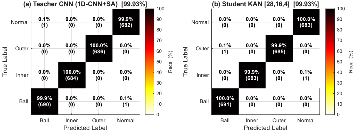
Fig. 12. Confusion matrices. Teacher 1D-CNN (left, 99.93%) and KAN student under VRM-KD (right, 99.93%) on the CWRU held-out test set (2,743 samples). Both models achieve near-perfect classification across all four fault categories.
