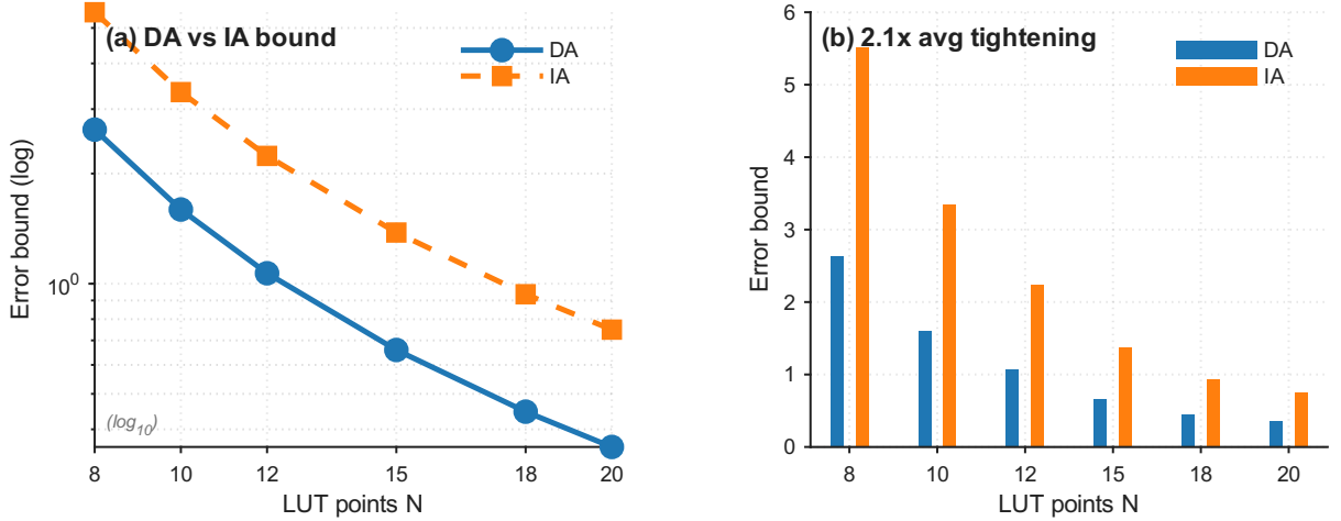
Fig. 9. DA vs. IA Bound Comparison with LUT Resolution. Left: DA achieves 2.1 \times tighter bounds than IA across all LUT resolutions ( N = 8\text{--}20 ), decreasing \propto 1/N^2 (Theorem C). At N=15 : DA = 0.66, IA = 1.38 (recomputed from the released checkpoint, 2026-08-03). Right: bar comparison. The gap follows from DA’s Galois-optimality (Theorem B).
