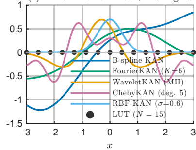
(f) All C^2 -BV families + LUT grid
