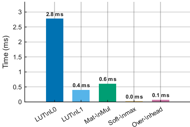
(b) Per-component WCET on S7-1200 Total = 3.86 ms (3.9% of 100 ms cycle)
