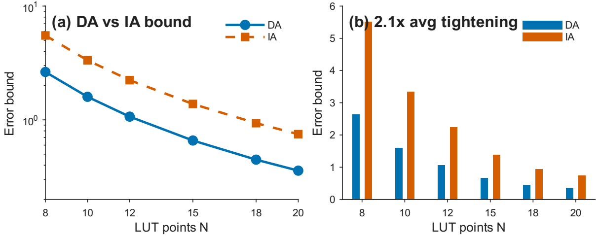
Fig. 9. DA vs. IA Bound Comparison with LUT Resolution. Left: DA achieves 2.1\times tighter bounds than IA across all LUT resolutions ( N = 8\text{--}20 ), decreasing \propto 1/N^2 (Theorem C). At N=15 : DA = 0.66, IA = 1.38 (recomputed from the released checkpoint, 2026-08-03). Right: bar comparison. The gap follows from DA’s Galois-optimality (Theorem B).
