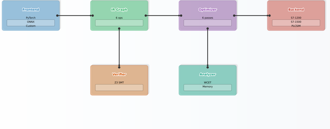
Fig. 6. Compiler architecture. Four-stage IR-based pipeline: Frontend (PyTorch \rightarrow IR) \rightarrow IR Graph (6 operation types) \rightarrow Optimizer (adaptive B-spline LUT) \rightarrow Backend (SCL code generation for S7-1200/S7-1500).
