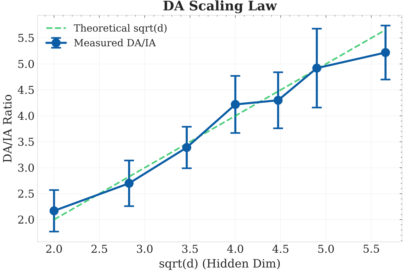
Fig. 8. DA/IA tightening ratio scaling law across 105 random KAN architectures [28, d, 4] . Left: scatter of 15 seeds per dimension with mean \pm 1\sigma overlaid; best-fit line ratio = 0.896\sqrt{d} + 0.349 , Pearson r = 0.987 ( p = 3.6 \times 10^{-5} ). Right: measured ratio vs. theoretical \sqrt{d} , confirming the random-walk mechanism of DA tightening. The trained KAN’s 3.1\times ratio ( d=16 ) lies at the 23rd percentile of its dimension group.
