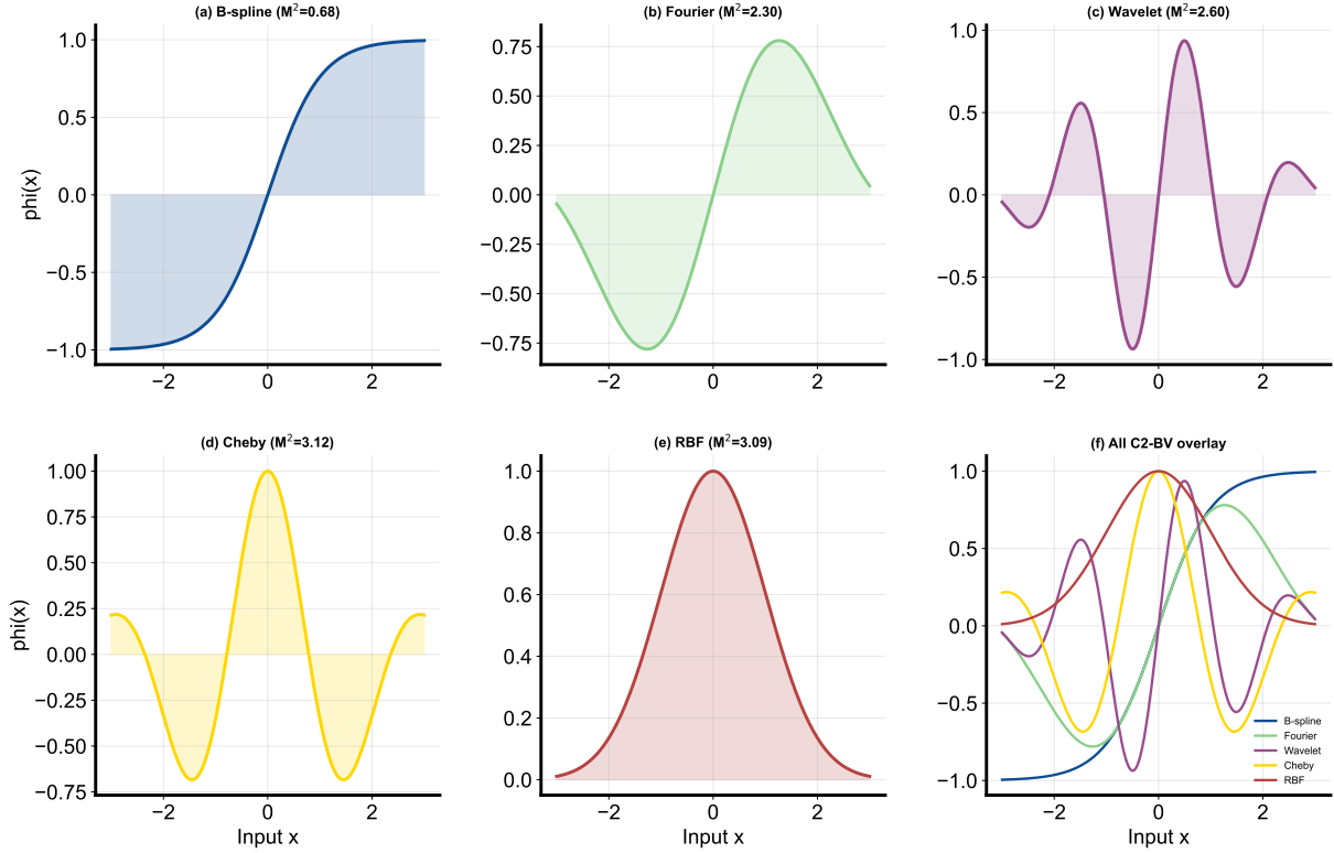
Fig. 1. C^2 -BV Architecture Family: Activation Basis Functions. Five SVNN-compliant activation function families on [-3, 3] with N=15 LUT grid points. All are C^2 with computable M_2 bounds (annotated per subplot). Despite diverse functional forms, all share the SVNN-critical property: each \phi_{j,i}(x_i) is a univariate C^2 function on a compact domain, enabling uniform LUT compilation with de Boor error bound M_2 h^2/8 (Theorem C).
