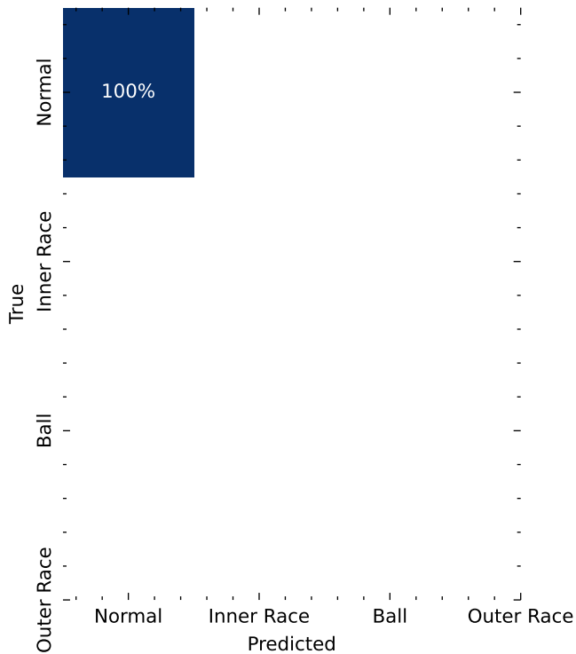
Teacher CNN
