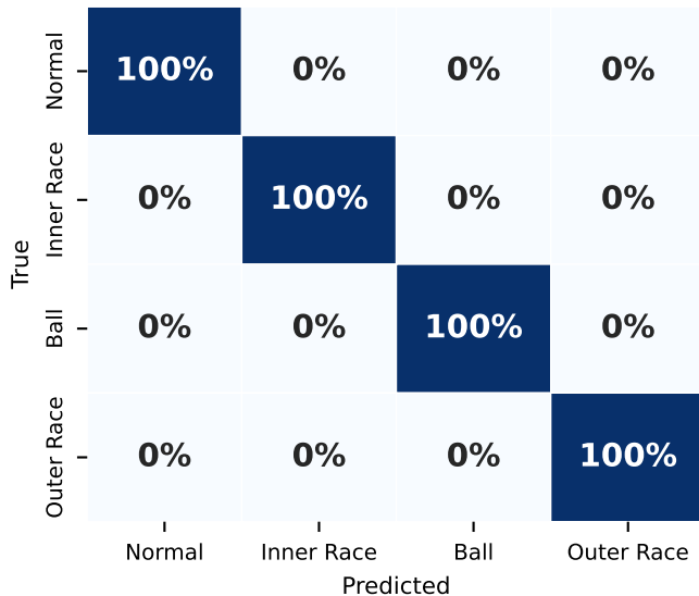
Teacher 1D-CNN (99.93%)
