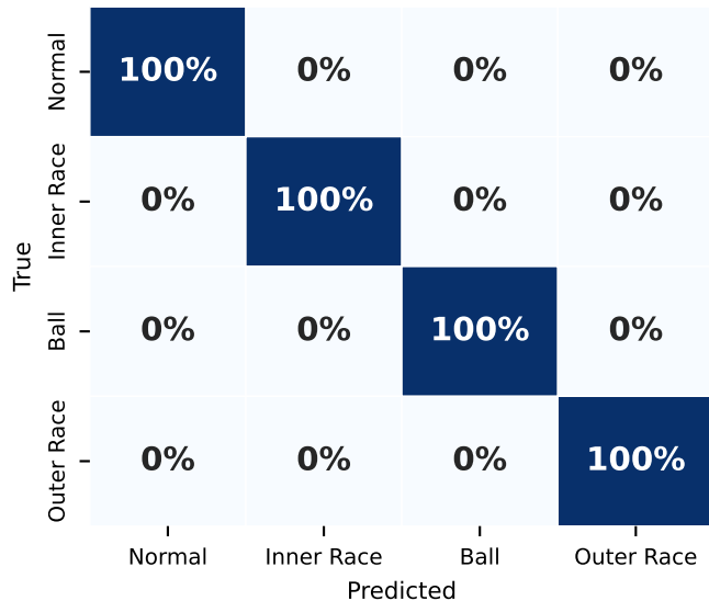
Student KAN VRM-KD (99.93%)
