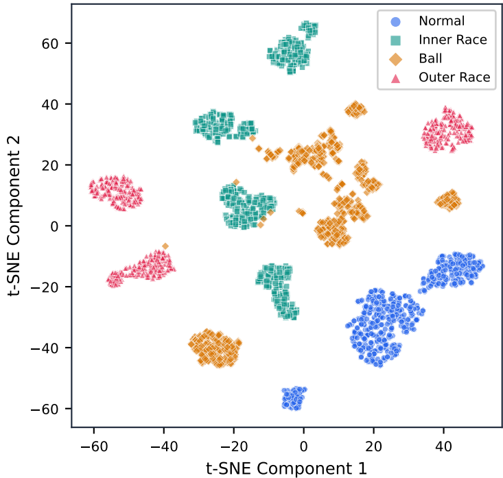
28-D Feature Space (t-SNE, Test Set, 2,743 samples)
