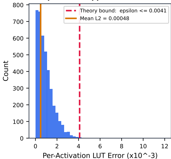
B-Spline LUT Approximation Error
