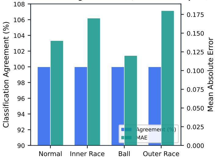
Per-Class: 100% Agreement (1,000 test samples)
