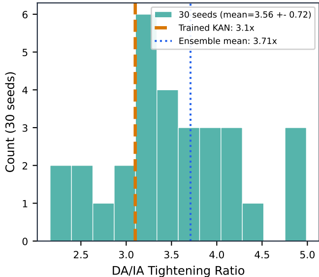
DA/IA Ratio Distribution ( d = 16 )
