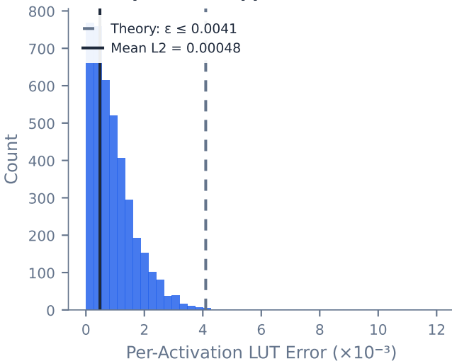
B-Spline LUT Approximation Error
