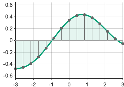
(e) RBF-KAN M_2=3.09
