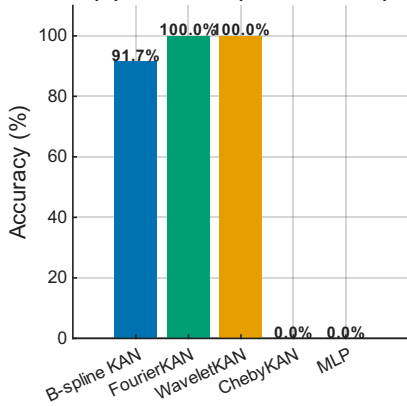
(b) XJTU-SY (domain shift)
