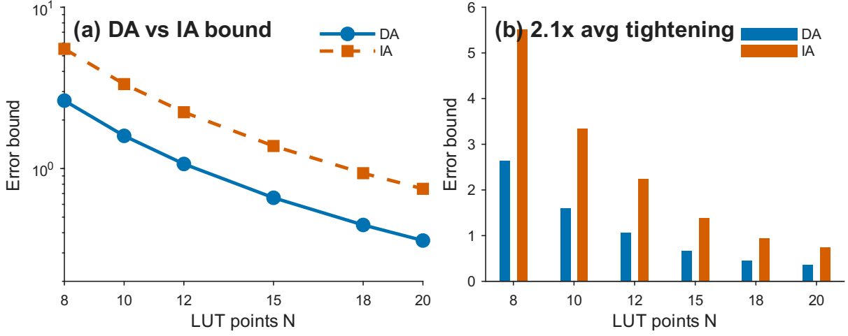
Fig. 9. DA vs. IA Bound Comparison with LUT Resolution. Left: DA achieves 2.1 \times tighter bounds than IA across all LUT resolutions ( N = 8\text{--}20 ), decreasing \propto 1/N^2 (Theorem C). At N=15 : DA = 0.66, IA = 1.38 (recomputed from the released checkpoint, 2026-08-03). Right: bar comparison. The gap follows from DA’s Galois-optimality (Theorem B).
