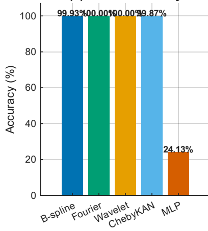
(b) CWRU Accuracy
