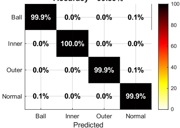
Teacher CNN (1D-CNN+SA) Accuracy = 99.89%
