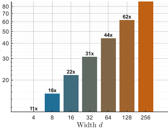
(b) MLP/KAN Ratio = \sqrt{d}/\gamma
