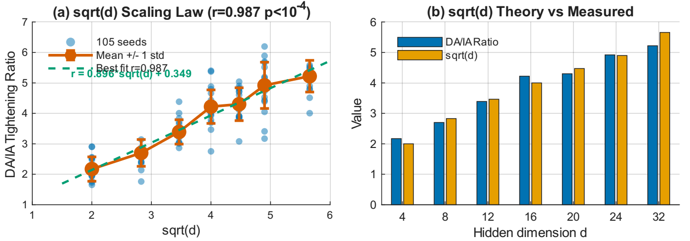
Fig. 8. DA/IA tightening ratio scaling law across 105 random KAN architectures [28, d , 4]. Left: scatter of 15 seeds per dimension with mean \pm 1\sigma overlaid; best-fit line ratio = 0.896\sqrt{d} + 0.349 , Pearson r = 0.987 ( p = 3.6 \times 10^{-5} ). Right: measured ratio vs. theoretical \sqrt{d} , confirming the random-walk mechanism of DA tightening. The trained KAN's 3.1\times ratio ( d=16 ) lies at the 23rd percentile of its dimension group.
