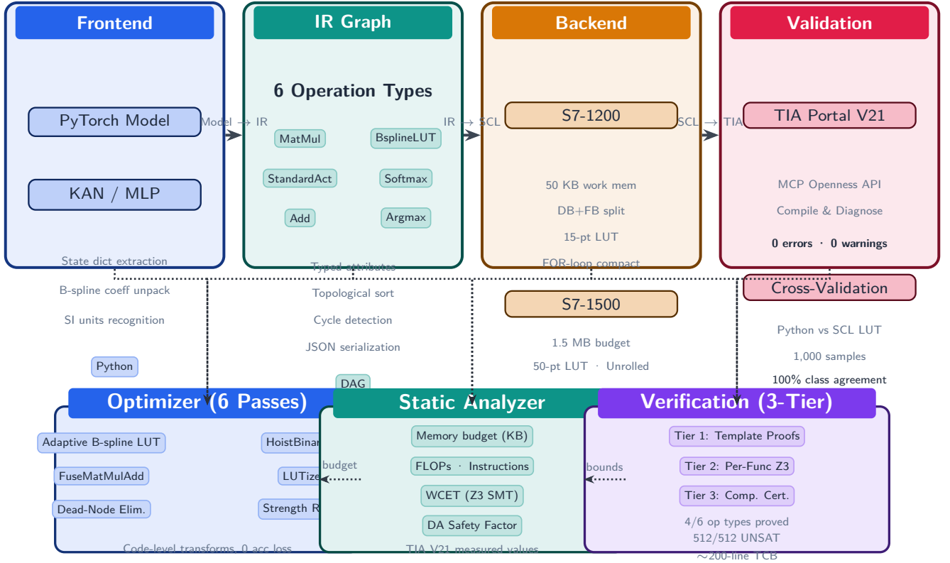
Fig. 6. Compiler architecture. Four-stage IR-based pipeline: Frontend (PyTorch \rightarrow IR) \rightarrow IR Graph (6 operation types) \rightarrow Optimizer (adaptive B-spline LUT) \rightarrow Backend (SCL code generation for S7-1200/S7-1500).
