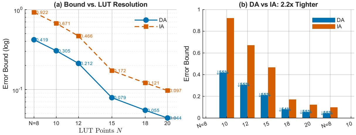
Fig. 9. DA vs. IA Bound Comparison with LUT Resolution. Left: DA achieves 2.2\times tighter bounds than IA across all LUT resolutions ( N = 8\text{--}20 ), decreasing \propto 1/N^2 (Theorem C). At N=15 : DA = 0.079, IA = 0.172. Right: bar comparison. The gap follows from DA's Galois-optimality (Theorem B).
