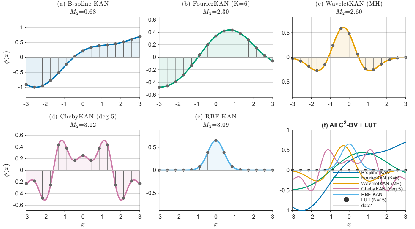
Fig. 11. C^2 -BV Architecture Family: representative activation basis functions with N=15 LUT grid points (vertical stems). Panel (a): B-spline KAN (cubic local basis, M_2 \approx 0.68 ); (b): FourierKAN ( \omega=0.4 , K=6 , M_2 \approx 2.30 ); (c): WaveletKAN (Mexican hat, M_2 \approx 2.60 ); (d): ChebyKAN (degree 5, M_2 \approx 3.12 ); (e): RBF-KAN ( \sigma=0.6 , M_2 \approx 3.09 ); (f): all five overlaid with N=15 LUT grid. The filled area under each curve illustrates that all C^2 -BV activations are positive on compact domains, enabling the universal discretization strategy of Proposition 5.
