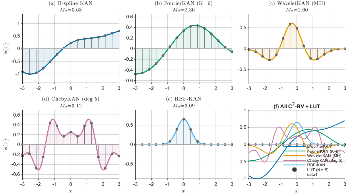
Fig. 1. C^2 -BV Architecture Family: Activation Basis Functions. Five SVNN-compliant activation function families on [-3, 3] with N=15 LUT grid points. All are C^2 with computable M_2 bounds (annotated per subplot). Despite diverse functional forms, all share the SVNN-critical property: each \phi_{j,i}(x_i) is a univariate C^2 function on a compact domain, enabling uniform LUT compilation with de Boor error bound M_2 h^2/8 (Theorem C).
