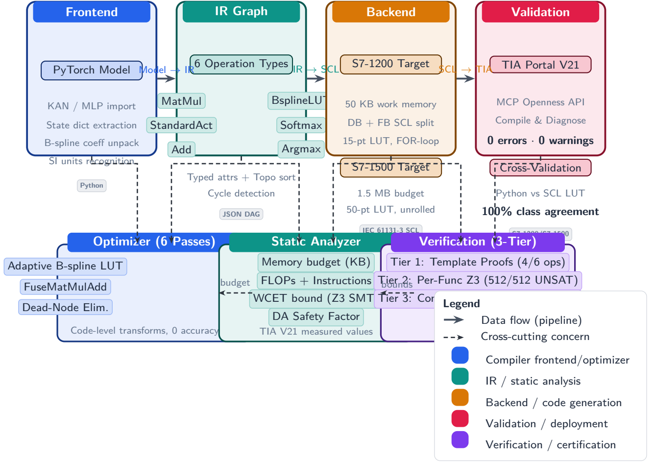
Fig. 6. Compiler architecture. Four-stage IR-based pipeline: Frontend (PyTorch → IR) → IR Graph (6 operation types) → Optimizer (adaptive B-spline LUT) → Backend (SCL code generation for S7-1200/S7-1500).
