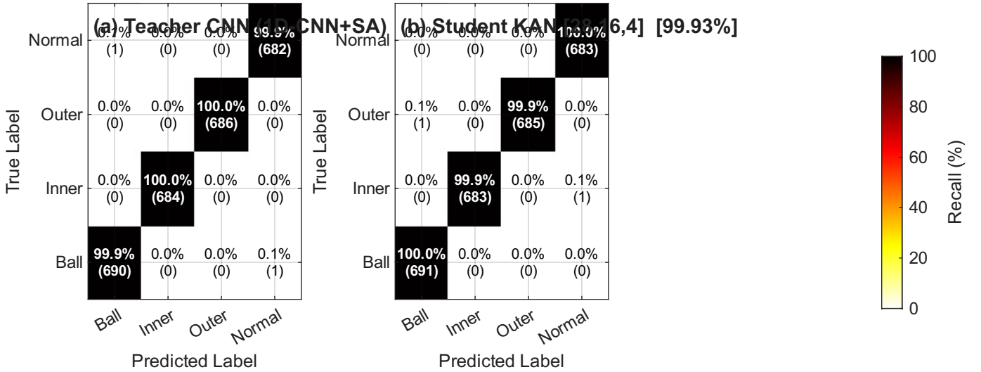
Fig. 12. Confusion matrices. Teacher 1D-CNN (left, 99.93%) and KAN student under VRM-KD (right, 99.93%) on the CWRU held-out test set (2,743 samples). Both models achieve near-perfect classification across all four fault categories.
